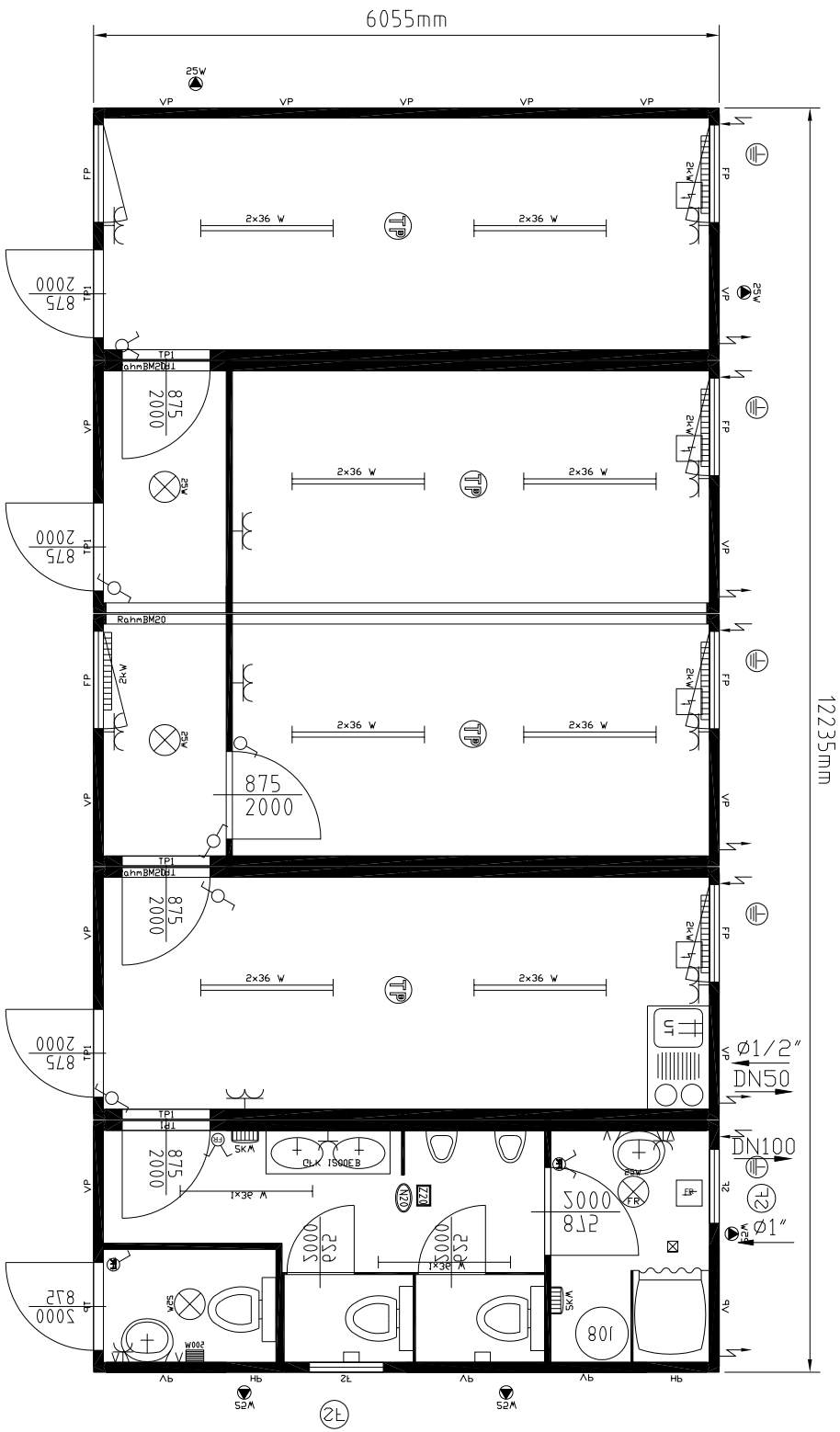
44602-001.dwg
